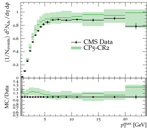
TransMAX charged-particle density \sqrt{s} = 13 TeV
