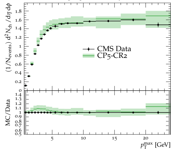
TransMAX charged-particle density \sqrt{s} = 13 TeV
