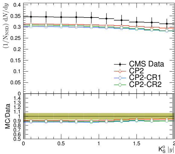
K_S^0 rapidity distribution, \sqrt{s} = 7 TeV
