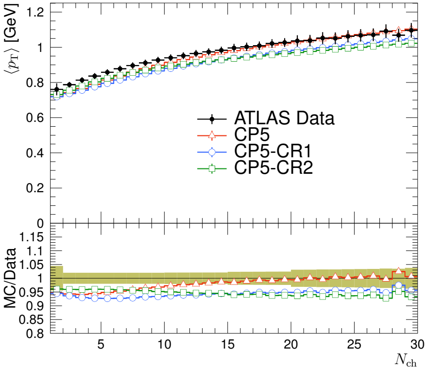
Transverse \langle p_T \rangle versus N_{\text{ch}} , \sqrt{s} = 7 TeV
