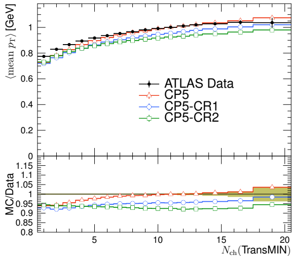
TransMIN, mean average transverse momentum, \sqrt{s} = 13 TeV
