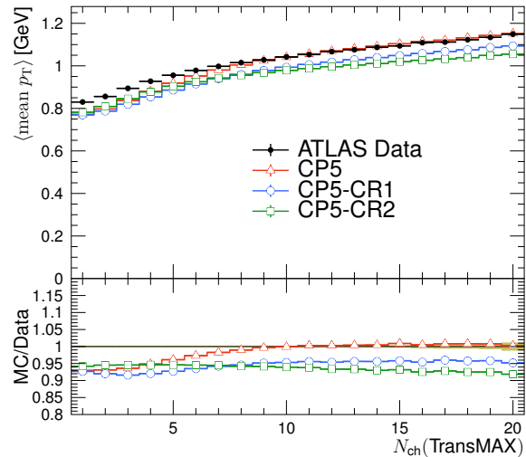
TransMAX, mean average transverse momentum, \sqrt{s} = 13 TeV
