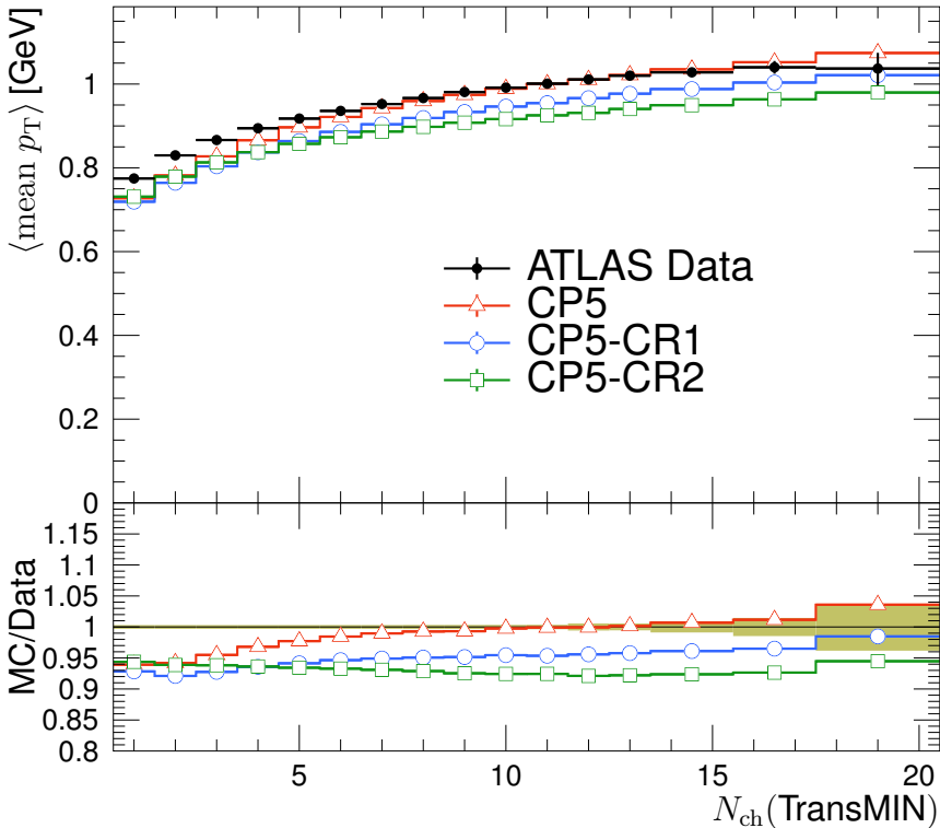
TransMIN, mean average transverse momentum, \sqrt{s} = 13 TeV
