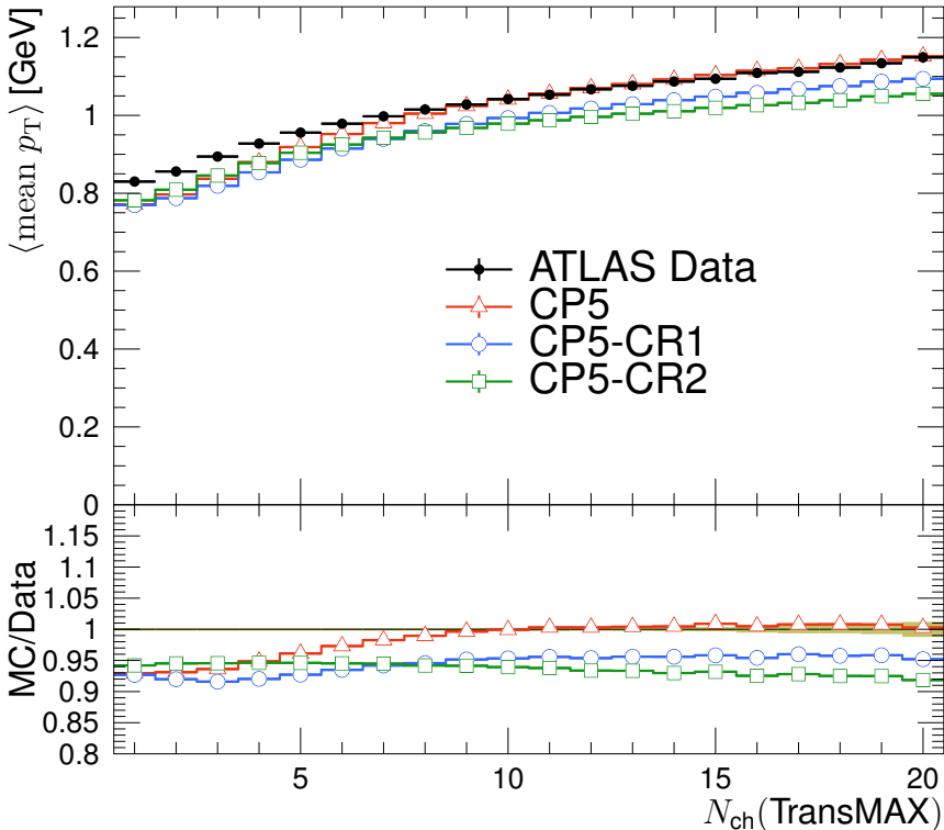
TransMAX, mean average transverse momentum, \sqrt{s} = 13 TeV
