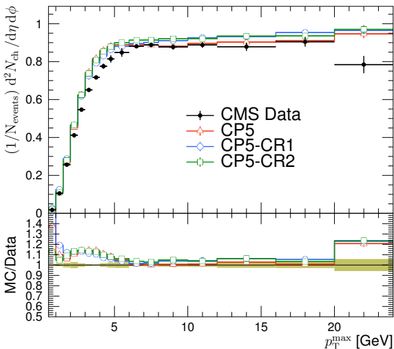
TransMAX charged-particle density \sqrt{s} = 13 TeV
