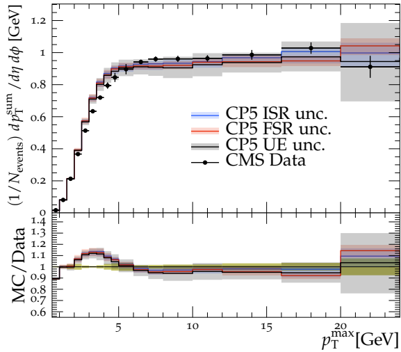
TransMIN charged p_T^{\text{sum}} density, \sqrt{s} = 13 TeV
