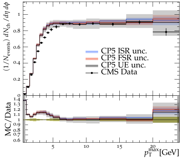
TransMIN charged-particle density, \sqrt{s} = 13 TeV
