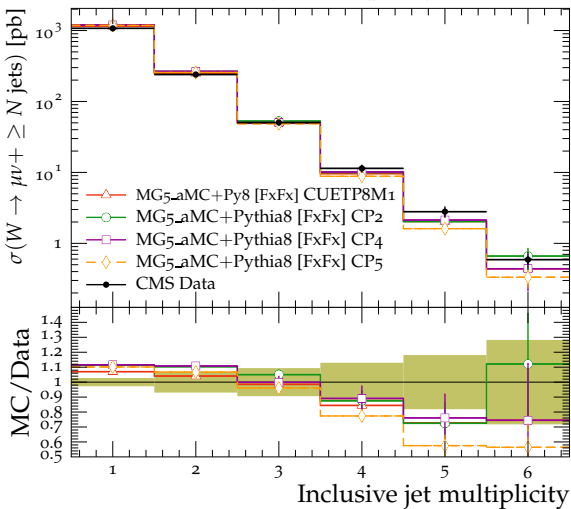
W+jets, inclusive jet multiplicity, \sqrt{s} = 13 TeV
