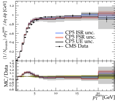
Transverse charged p_T^{\text{sum}} density \sqrt{s} = 13 TeV
