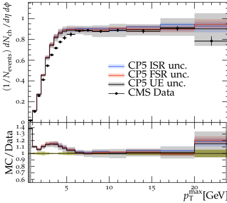
Transverse charged-particle density \sqrt{s} = 13 TeV
