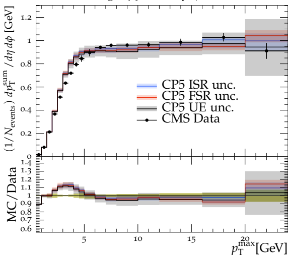
TransMAX charged p_T^{\text{sum}} density, \sqrt{s} = 13 TeV
