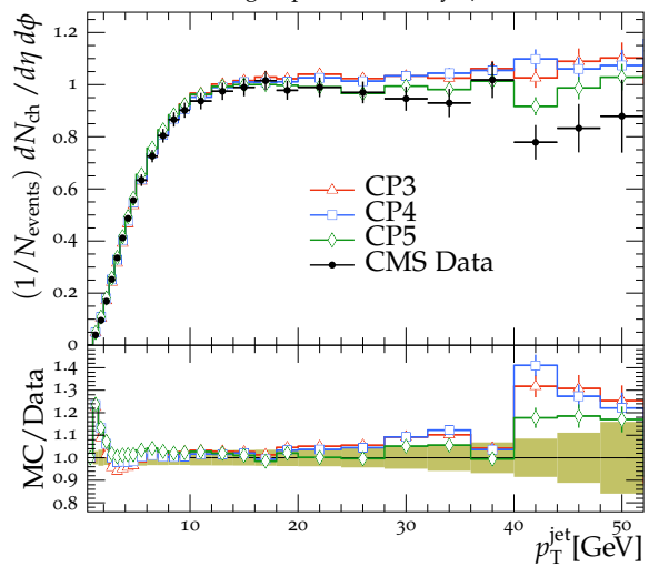
TransMIN charged-particle density, \sqrt{s} = 13 TeV
