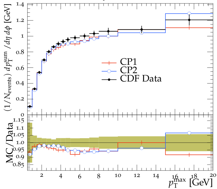
TransMAX charged p_T^{\text{sum}} density, \sqrt{s} = 1.96 TeV
