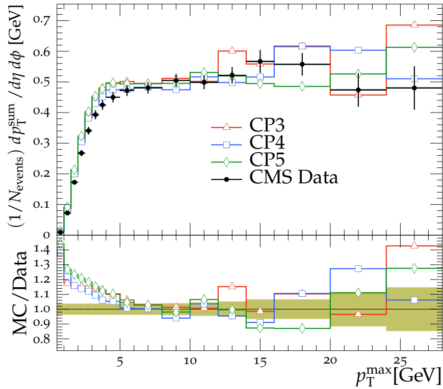
TransMIN charged p_T^{\text{sum}} density, \sqrt{s} = 7 \text{ TeV}
