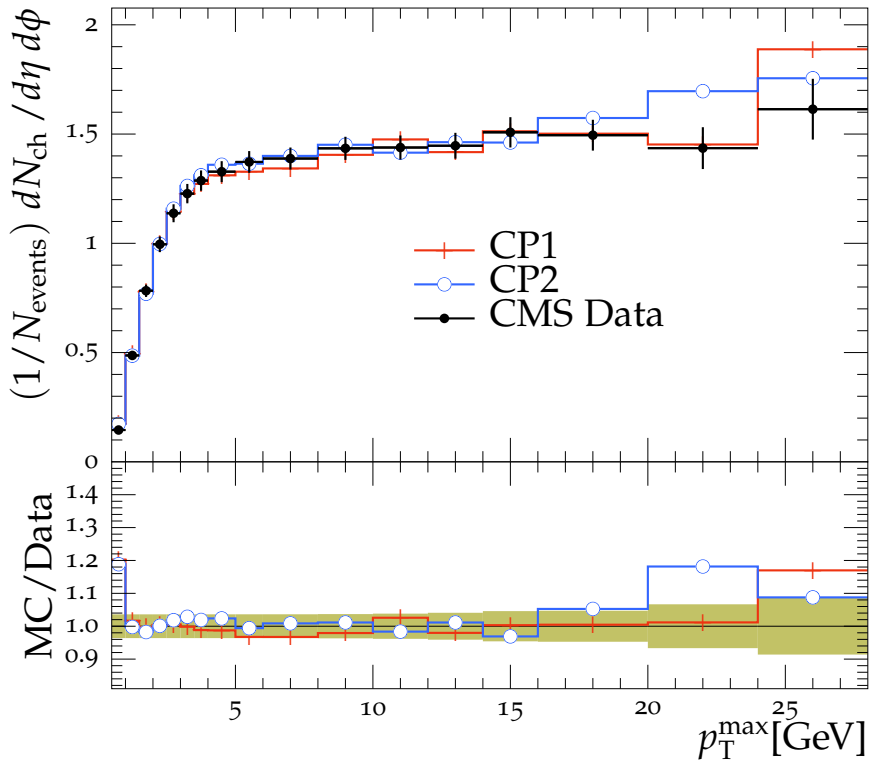
TransMAX charged-particle density, \sqrt{s} = 7 TeV
