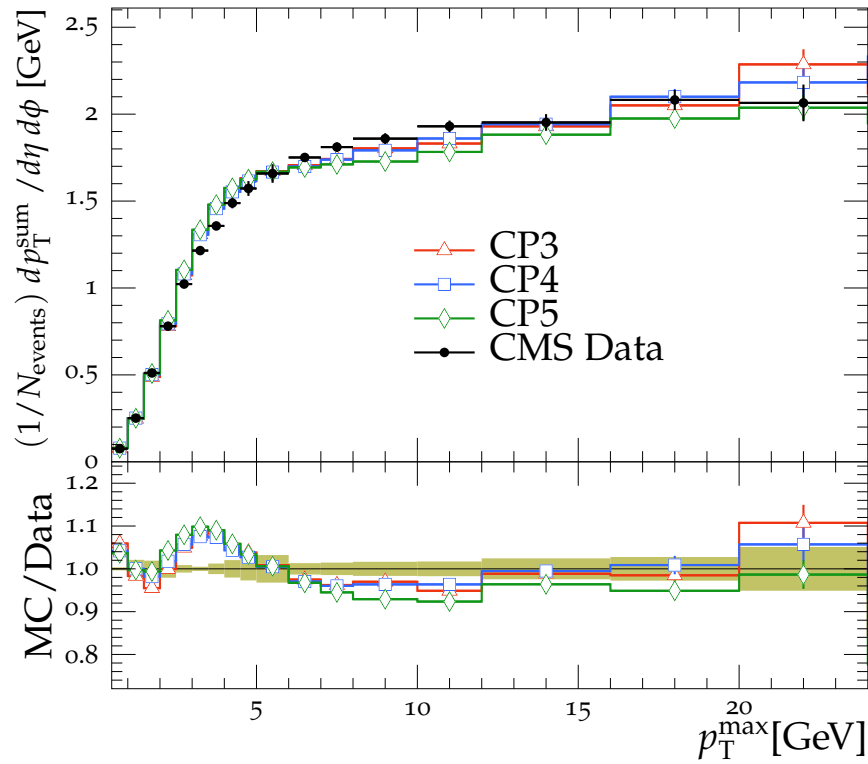
TransMAX charged p_T^{\text{sum}} density, \sqrt{s} = 13 \text{ TeV}
