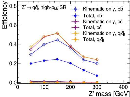
CMS Simulation (13 TeV)
