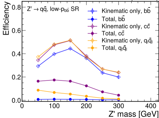
CMS Simulation (13 TeV)
