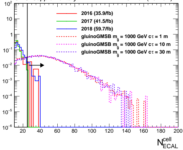
CMS Supplementary 137 fb -1 (13 TeV)
