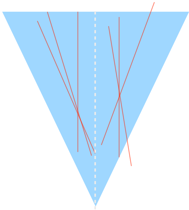
AK8 jet
