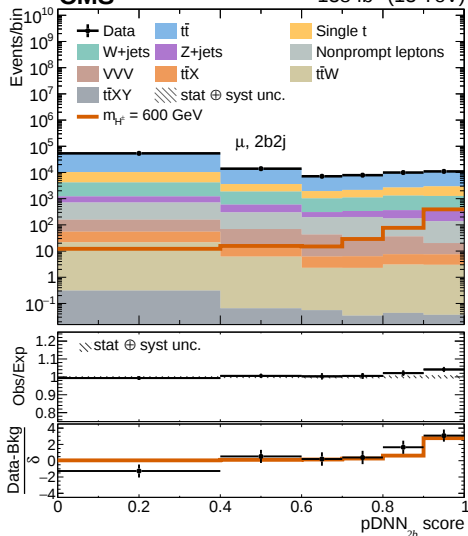
CMS 138 fb -1 (13 TeV)
