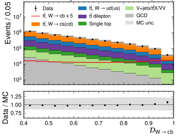
CMS Preliminary 138 fb -1 (13 TeV)
