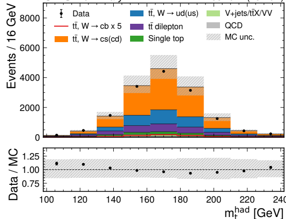
CMS Preliminary 138 fb -1 (13 TeV)
