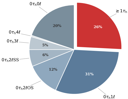
(a) Four top quarks decay channels.
