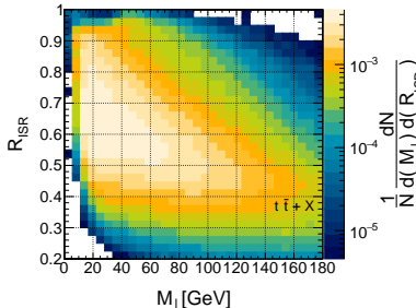
CMS Simulation Preliminary Region 0L J X
