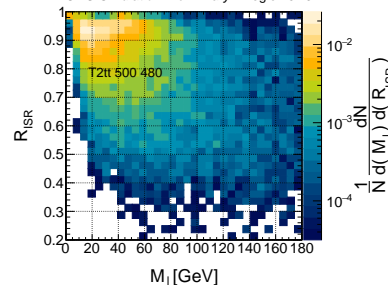
CMS Simulation Preliminary Region 2L J X
