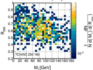
CMS Simulation Preliminary Region 2L J X
