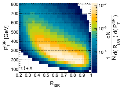
CMS Simulation Preliminary Region 0L J X
