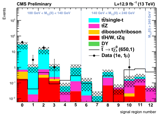
(b) e\mu channel
