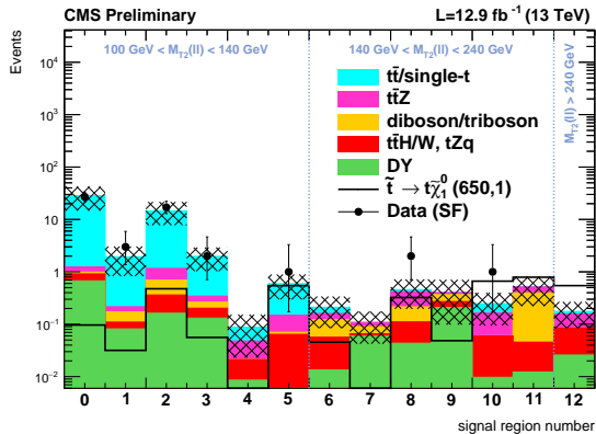
(a) \mu\mu and ee channel
