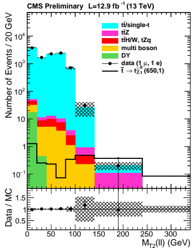
(c) e\mu channel
