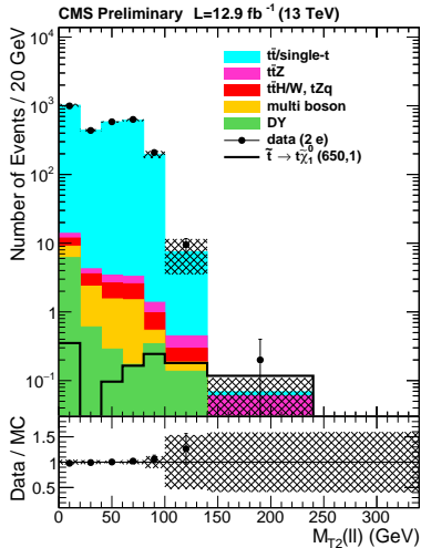
(b) ee channel
