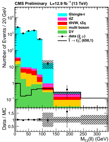
(a) \mu\mu channel
