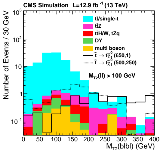
(c) M_{T_2}(blbl)
