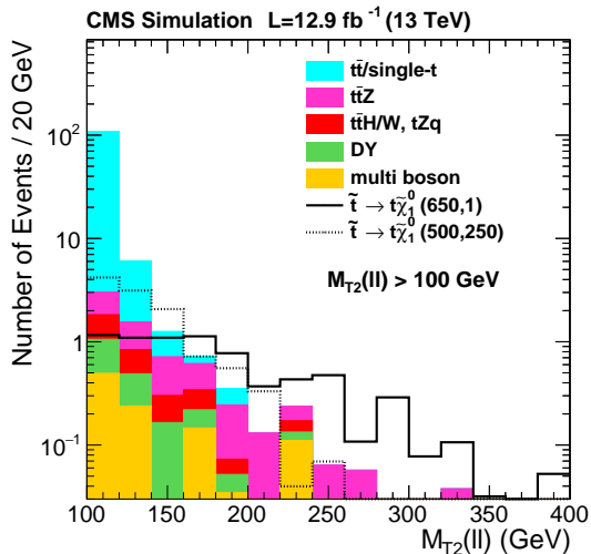
(a) M_{T_2}(\ell\ell)
