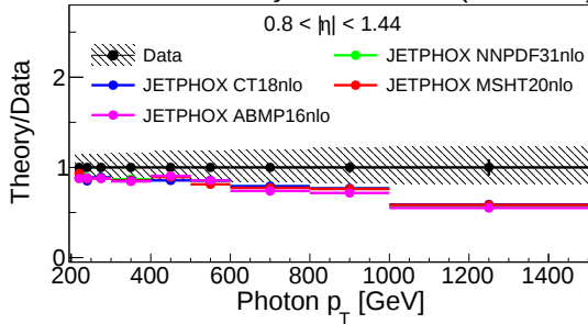
CMS Preliminary 27 fb -1 (13.6 TeV)
