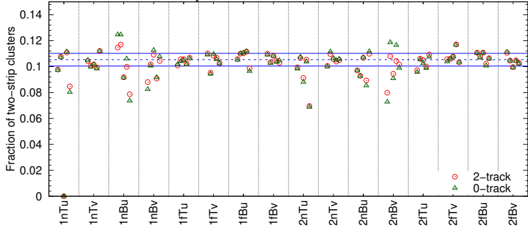
CMS-TOTEM Preliminary
