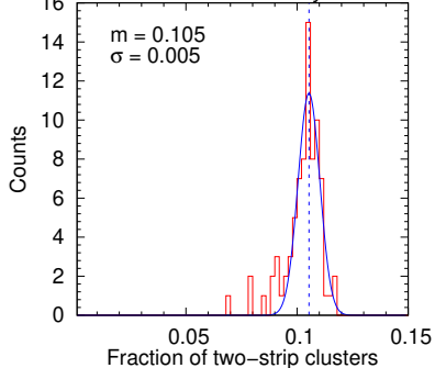
CMS-TOTEM Preliminary
