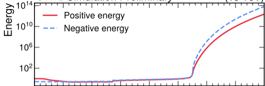
CMS Simulation Preliminary (13 TeV)
