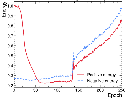
CMS Simulation Preliminary (13 TeV)
