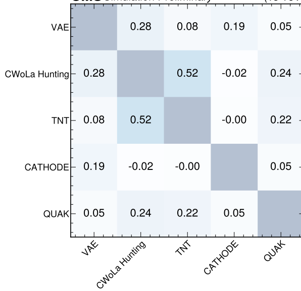
CMS Simulation Preliminary (13 TeV)
