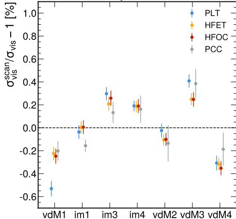
CMS Preliminary Fill 6868 (2018, 13 TeV)
