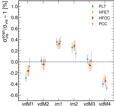
CMS Preliminary Fill 6016 (2017, 13 TeV)
