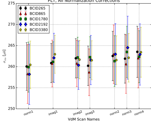
PLT, All Normalization Corrections
