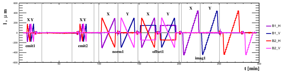
DOROS beams position in VdM Scan with Fill6868 (Take 2)
