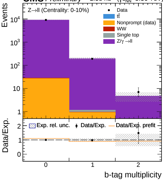
CMS Preliminary 1.58 \text{ nb}^{-1} (\sqrt{s_{\text{NN}}}=5.36 \text{ TeV})
