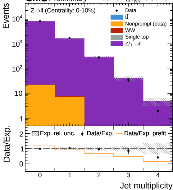
CMS Preliminary 1.58 \text{ nb}^{-1} (\sqrt{s_{\text{NN}}}=5.36 \text{ TeV})
