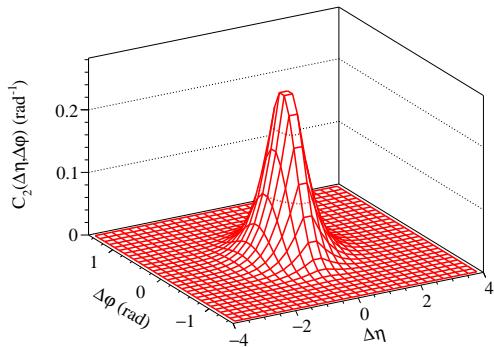
Fit function:: Near-side peak
