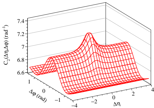
Fit function:: Flow background
