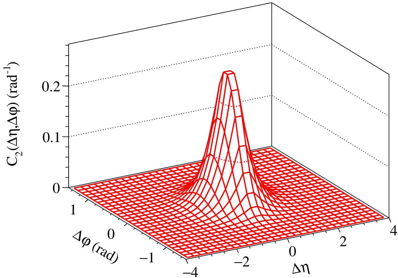
Fit function:: Near-side peak
