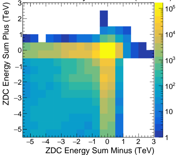
CMS Preliminary 2023 PbPb (5.36 TeV)
