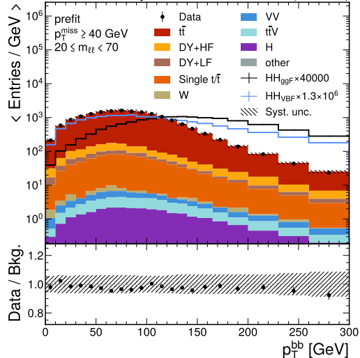
CMS Preliminary 62 fb -1 (13.6 TeV)
