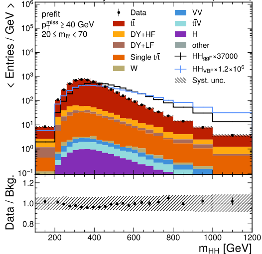
CMS Preliminary 62 fb -1 (13.6 TeV)
