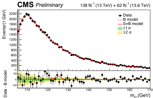
(c) ggF 3
