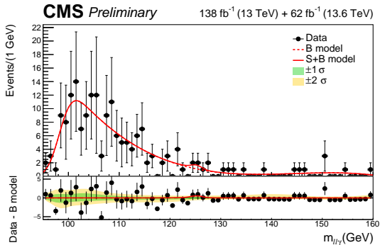
(a) ggF 1
