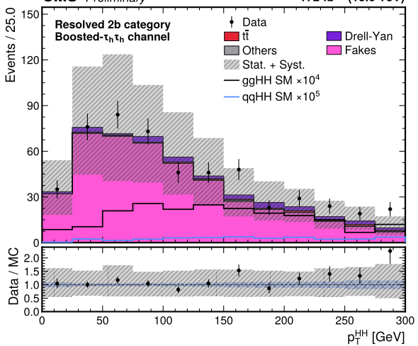
CMS Preliminary 172 fb -1 (13.6 TeV)
