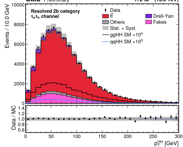
CMS Preliminary 172 fb -1 (13.6 TeV)
