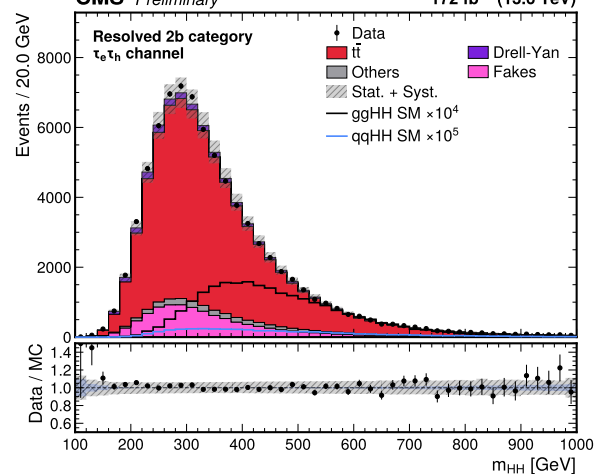
CMS Preliminary 172 \text{ fb}^{-1} (13.6 TeV)
