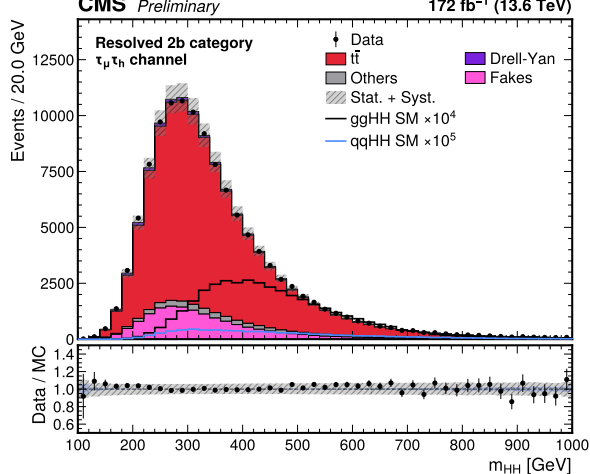
CMS Preliminary 172 \text{ fb}^{-1} (13.6 TeV)
