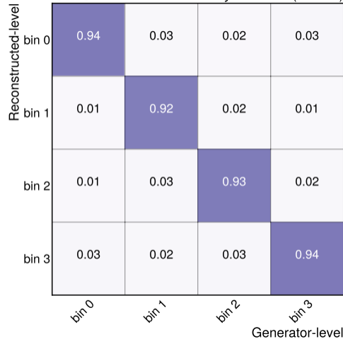
CMS Simulation Preliminary (13 TeV)
