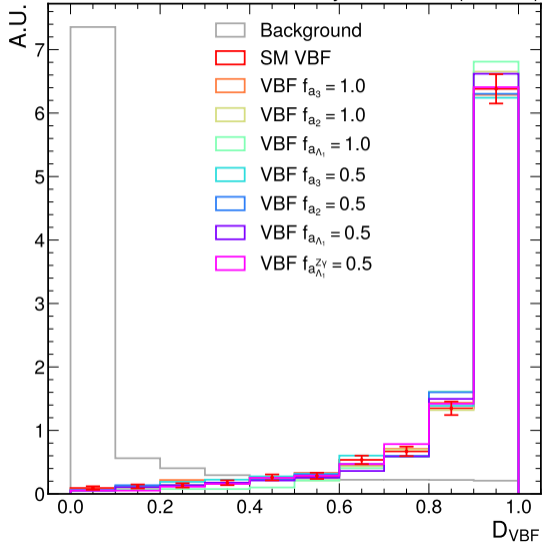
CMS Simulation Preliminary (13 TeV)
