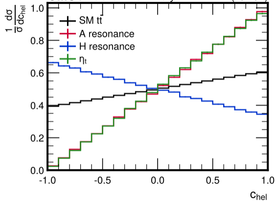
CMS Simulation Preliminary (13 TeV)
