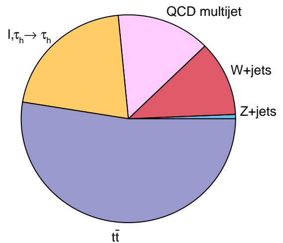
\mu\tau_h B-tag Loose- m_T
