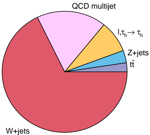
\mu\tau_h No B-tag Loose- m_T
