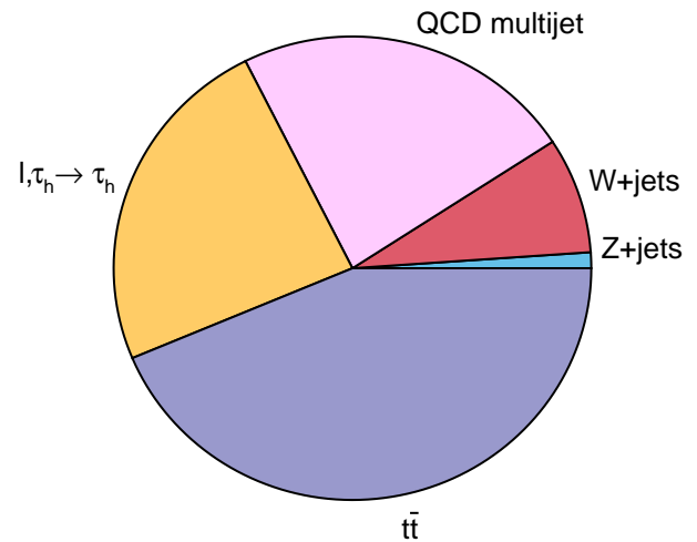
\mu\tau_h B-tag Tight- m_T
