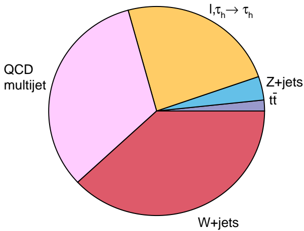
\mu\tau_h No B-tag Tight- m_T
