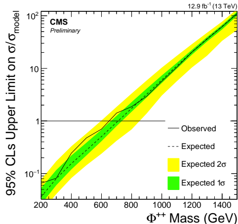
(b) 100% \mu\tau
