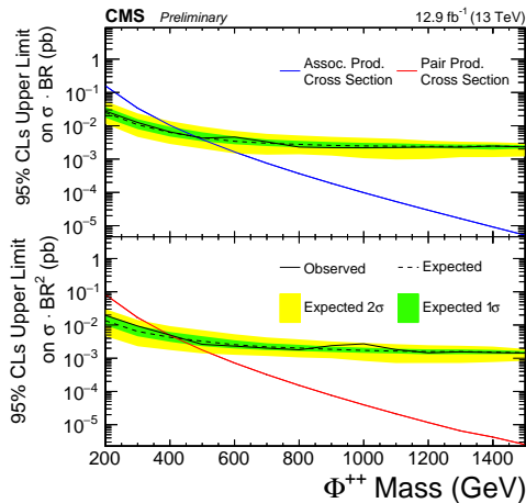
(c) 100% \tau\tau
