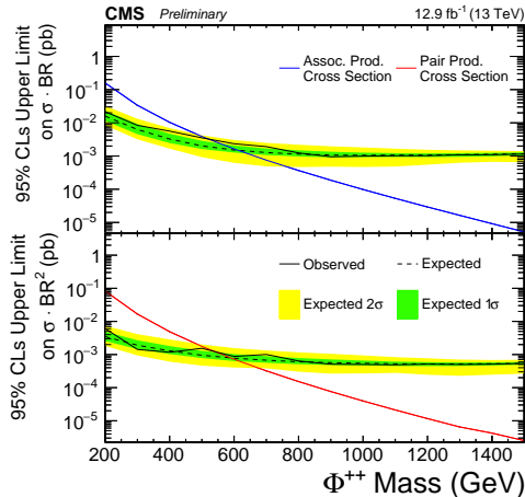
(a) 100% \mu\tau
