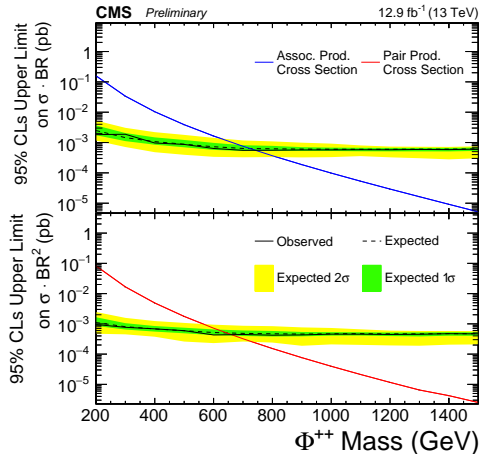
(a) 100% ee
