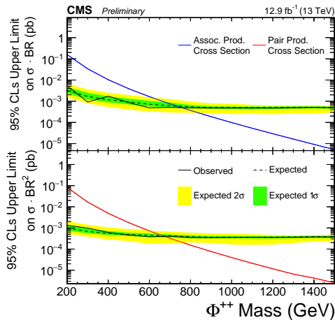
(c) 100% e\mu
