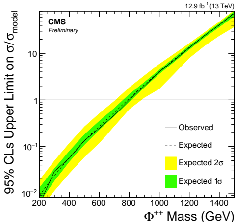
(b) 100% ee
