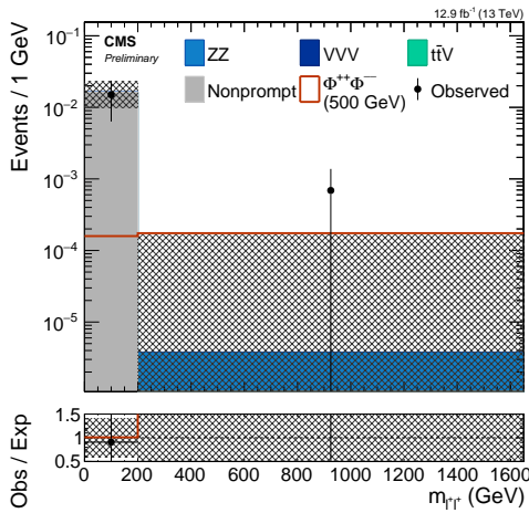
(c) l^\pm l^\pm \tau^\pm \tau^\pm \tau^\pm
