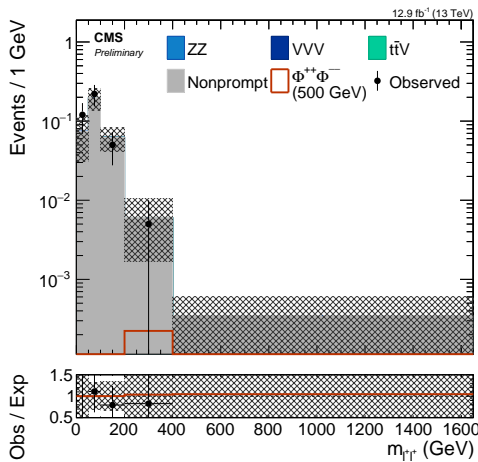
(e) l^\pm \tau^\pm \tau^\pm \tau^\pm
