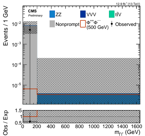
(f) \tau^\pm \tau^\pm \tau^\pm \tau^\pm
