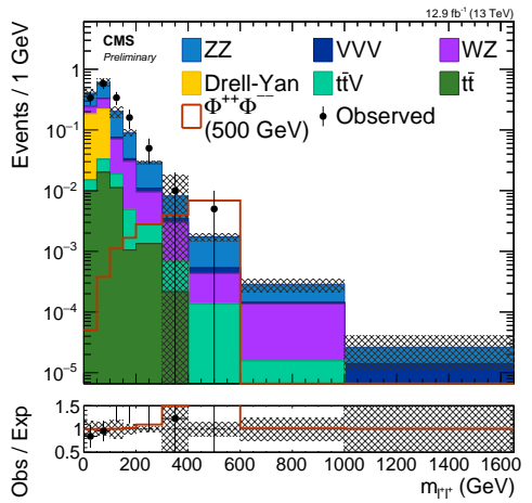
(b) l^\pm l^\pm l^\pm \tau^\pm \tau^\pm
