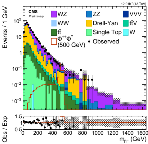
(a) l^\pm l^\pm l^\mp
