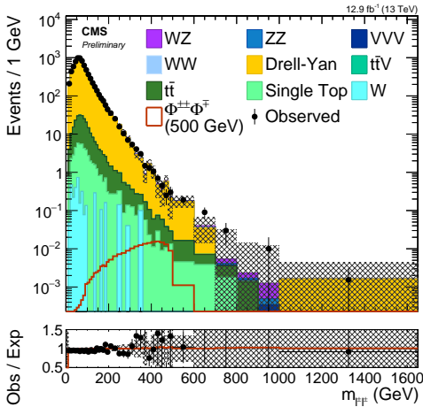
(c) l^\pm \tau^\pm l^\mp
