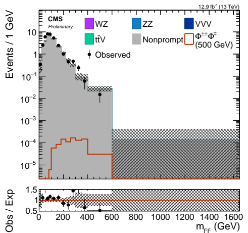
(f) \tau^\pm \tau^\pm \tau^\mp
