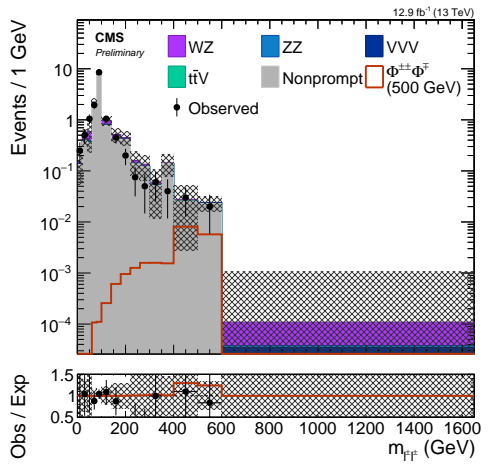
(b) l^\pm l^\pm \tau^\mp
