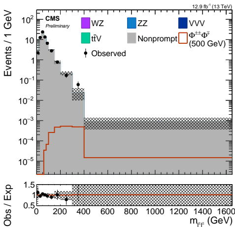
(e) \tau^\pm \tau^\pm l^\mp
