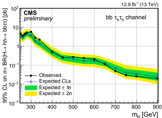
(c) bb \tau_h\tau_h
