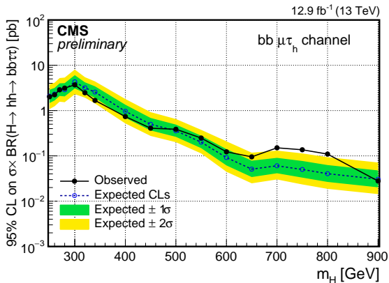
(a) bb \mu\tau_h
